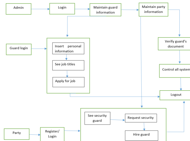
Fig: System Architecture Diagram
